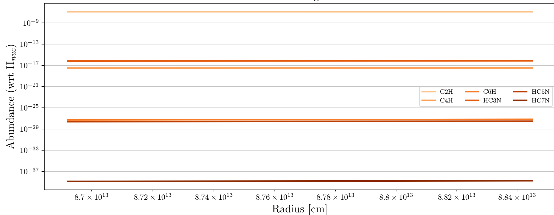
Particle 49706 - Daughter Molecules
